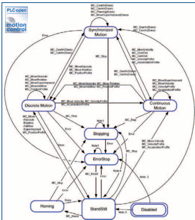
PLCopen State-Diagramm
